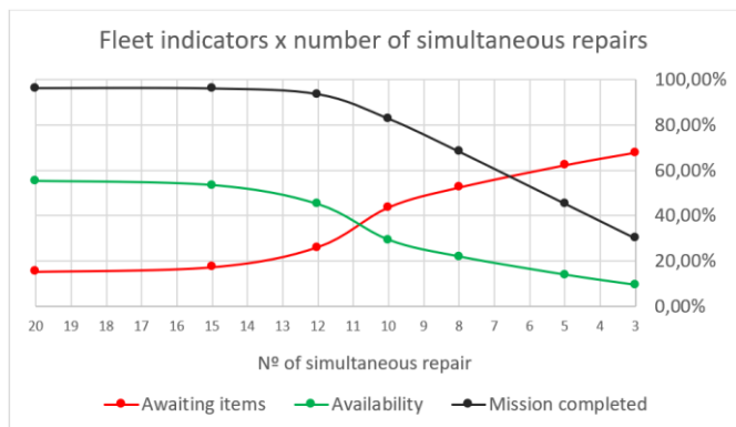
Fig. 7: Impact of simultaneous repair in fleet indicators
